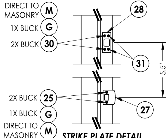
STRIKE PLATE DETAIL
