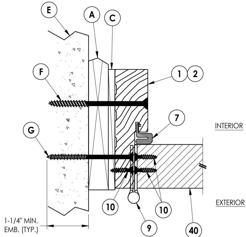
1 8 HORIZONTAL CROSS SECTION Outswing Shown (Inswing Similar) Shown w/ 1X Buck
