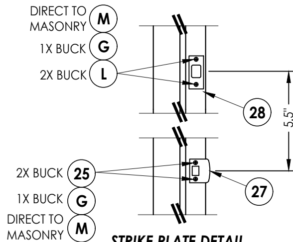
STRIKE PLATE DETAIL
