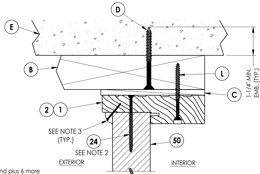
5 VERTICAL CROSS SECTION 7 Outswing Shown (Inswing Similar) Shown w/ 2X Buck
