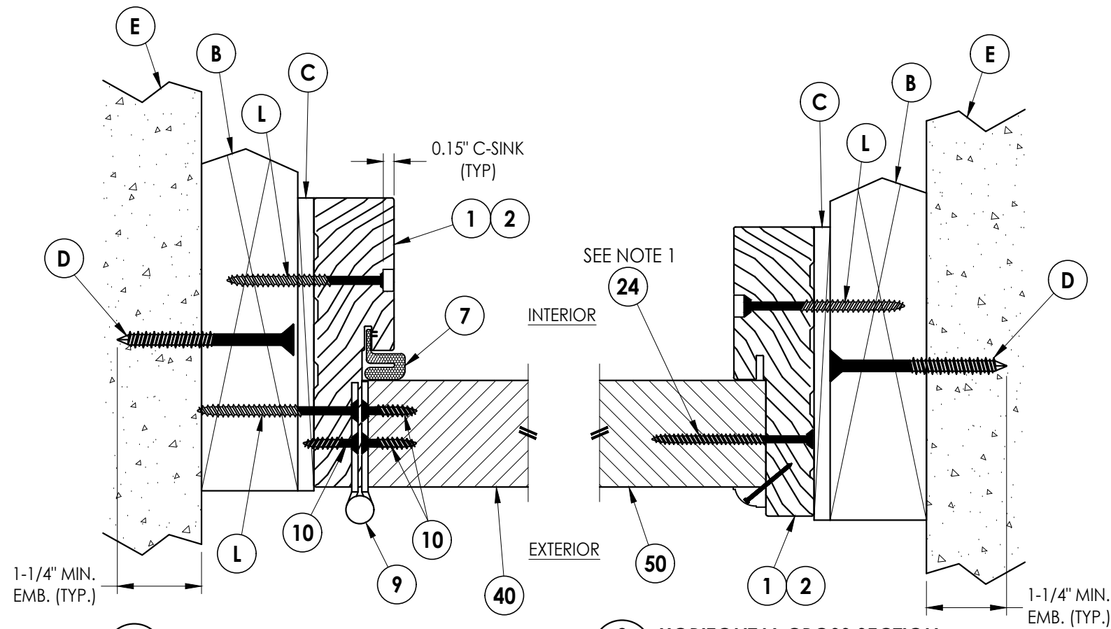
1 HORIZONTAL CROSS SECTION 7 Outswing Shown (Inswing Similar) Shown w/ 2X Buck
