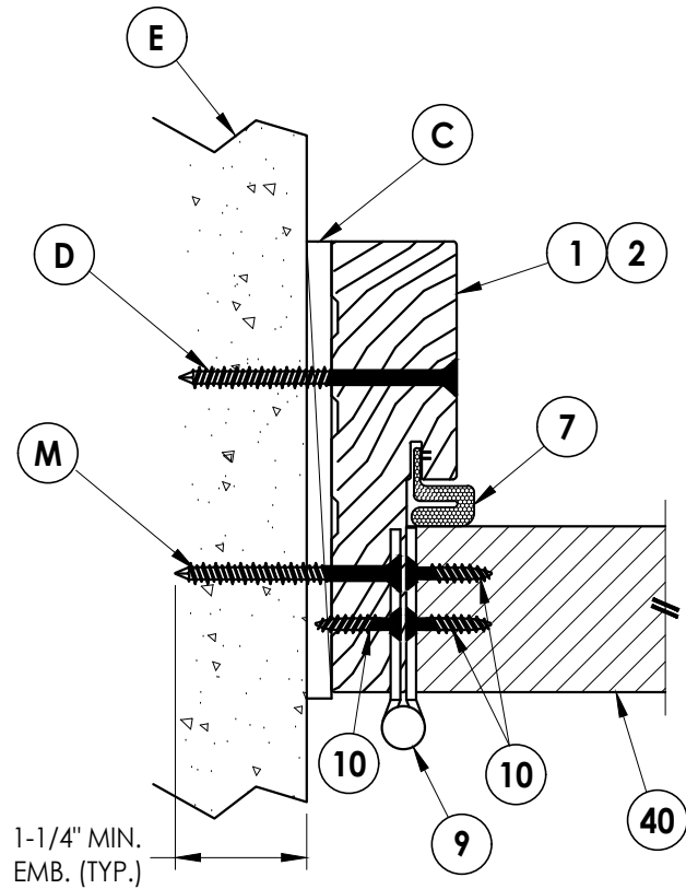
1 9 HORIZONTAL CROSS SECTION Outswing Shown (Inswing Similar) Shown Direct to Masonry
