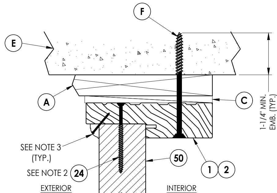
5 8 VERTICAL CROSS SECTION Outswing Shown (Inswing Similar) Shown w/ 1X Buck
