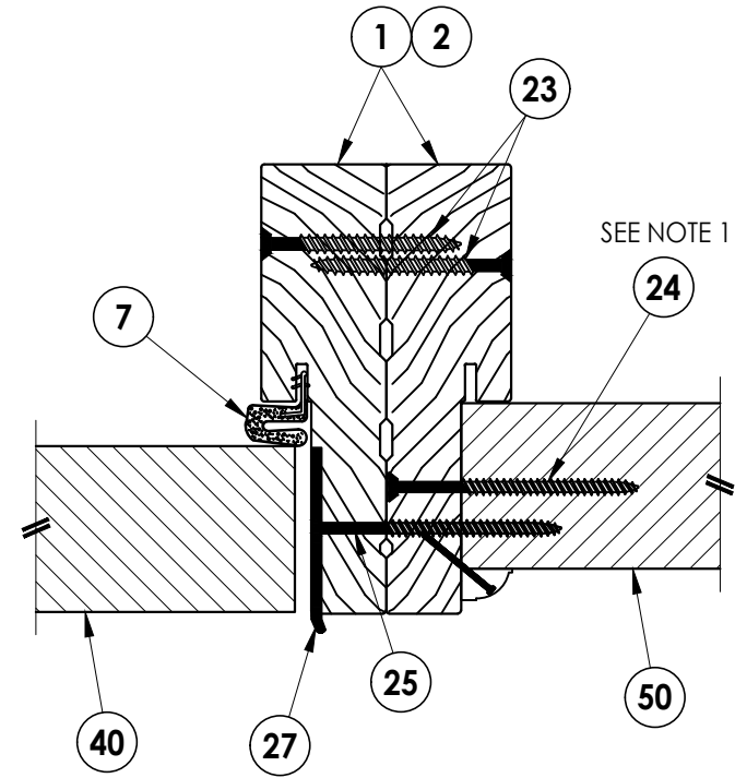
2 HORIZONTAL CROSS SECTION 6 Outswing Shown (Inswing Similar)
