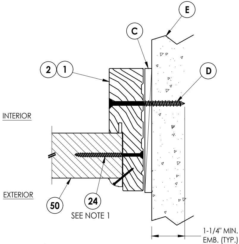
2 9 HORIZONTAL CROSS SECTION Outswing Shown (Inswing Similar) Shown Direct to Masonry
