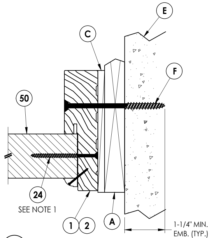
2 8 HORIZONTAL CROSS SECTION Outswing Shown (Inswing Similar) Shown w/ 1X Buck
