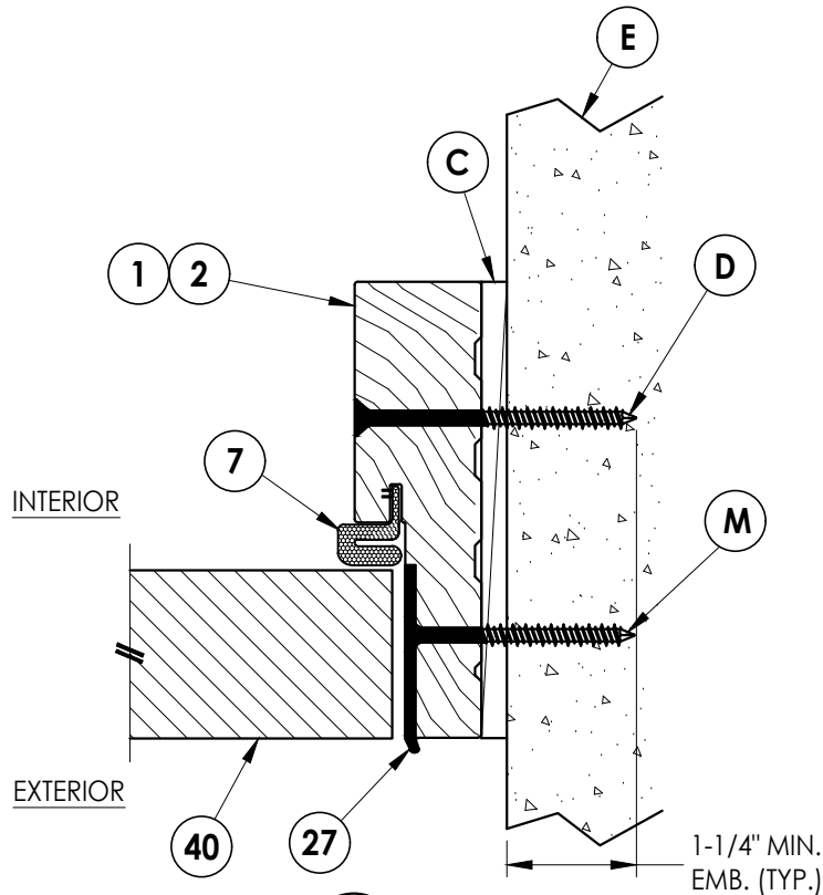
3 9 HORIZONTAL CROSS SECTION Outswing Shown (Inswing Similar) Shown Direct to Masonry
